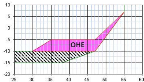
4-pipe configuration - Extended operating range with OHE kit
