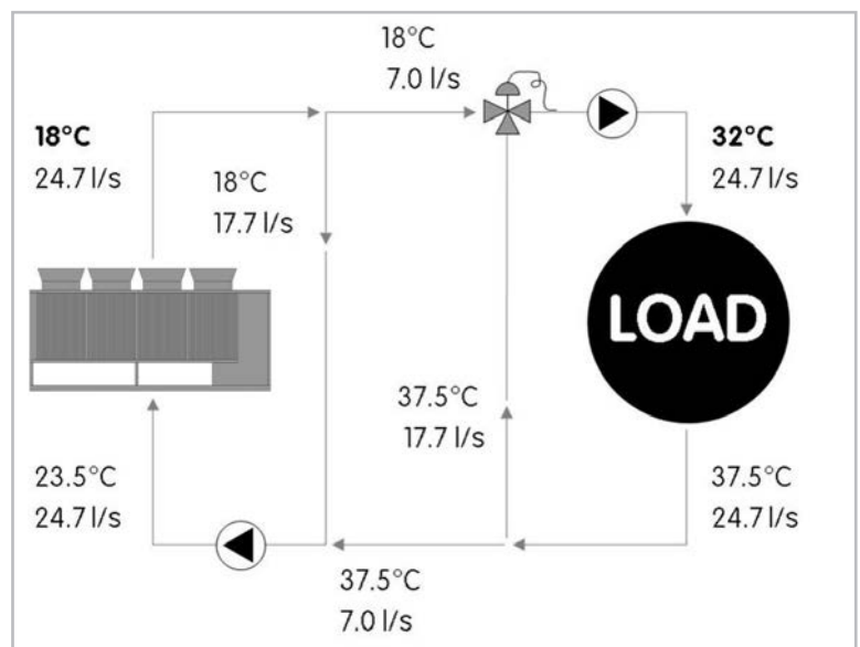
Example referred to WSAN-XSC3 MF 200.4 SC EXCELLENCE version. Appropriate supply water temperature for the correct unit operation. Nominal water flow rate.
