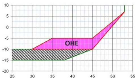
2-pipe configuration - Extended operating range with OHE kit
